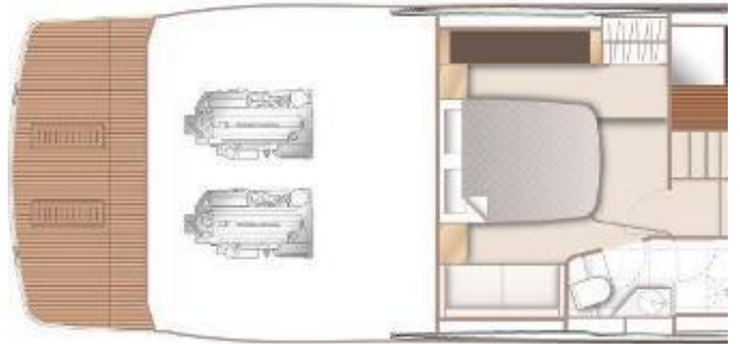
Princess V50 Lower Deck Layout Plan
